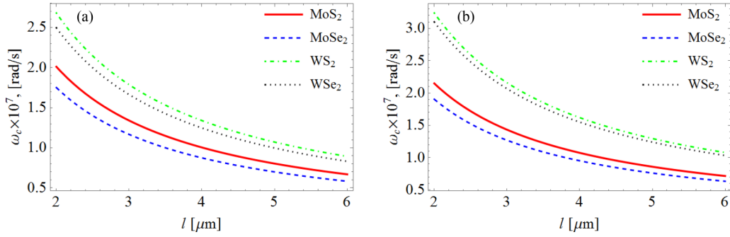
FIG. 2. The dependence of the cyclotron frequency \omega_c on the parameter l , determined by the distance between the counterpropagating laser beams. Calculations performed for |k_1| + |k_2| = 3 \mu\text{m}^{-1} . (a) and (b) \omega_c as a function of l for A and B polaritons, respectively.
